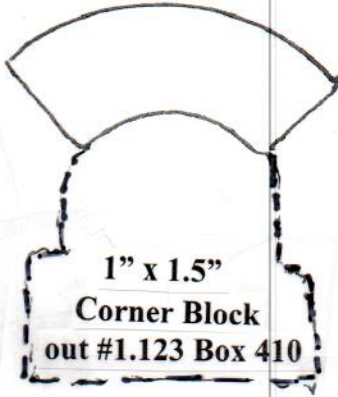
1" x 1.5"
